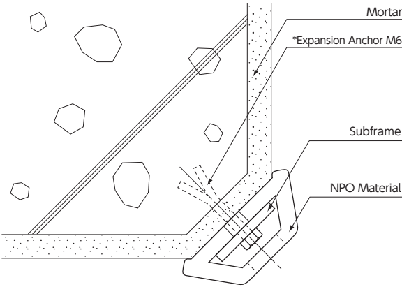
RC Foundation + Mortar
