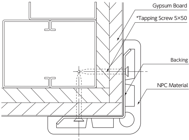
LGS Foundation + Gypsum board(Double Layer)
