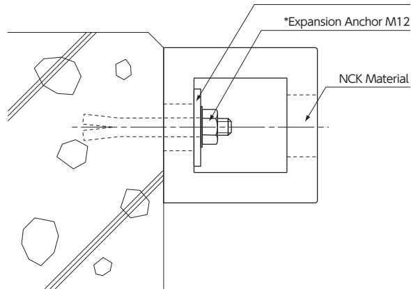
RC Wall
