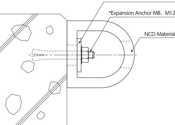
RC Wall
