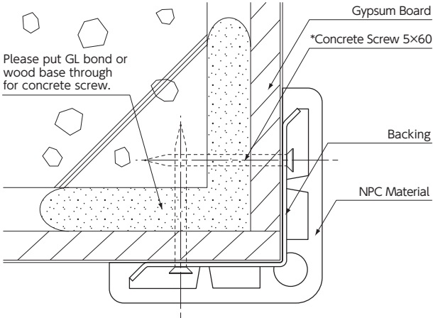
RC Foundation + GL Construction Method
