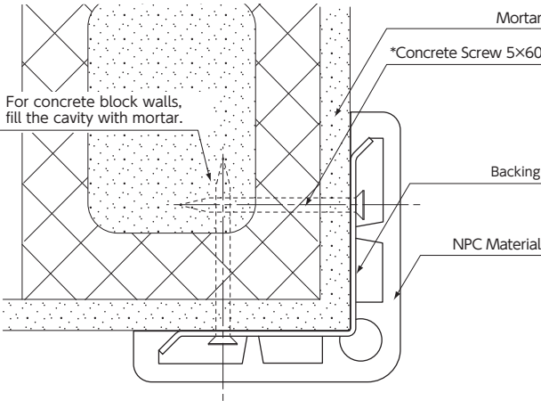
CB Foundation + Mortar
